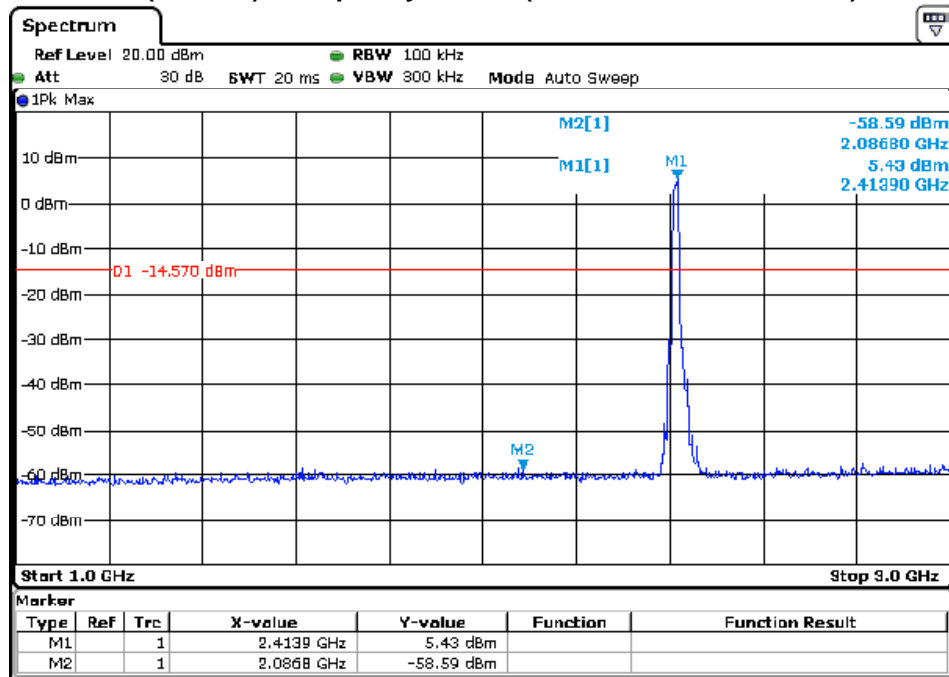
CH 1 (B mode) - Frequency Band 2 (1000 MHz < f \leq 3000 MHz)
