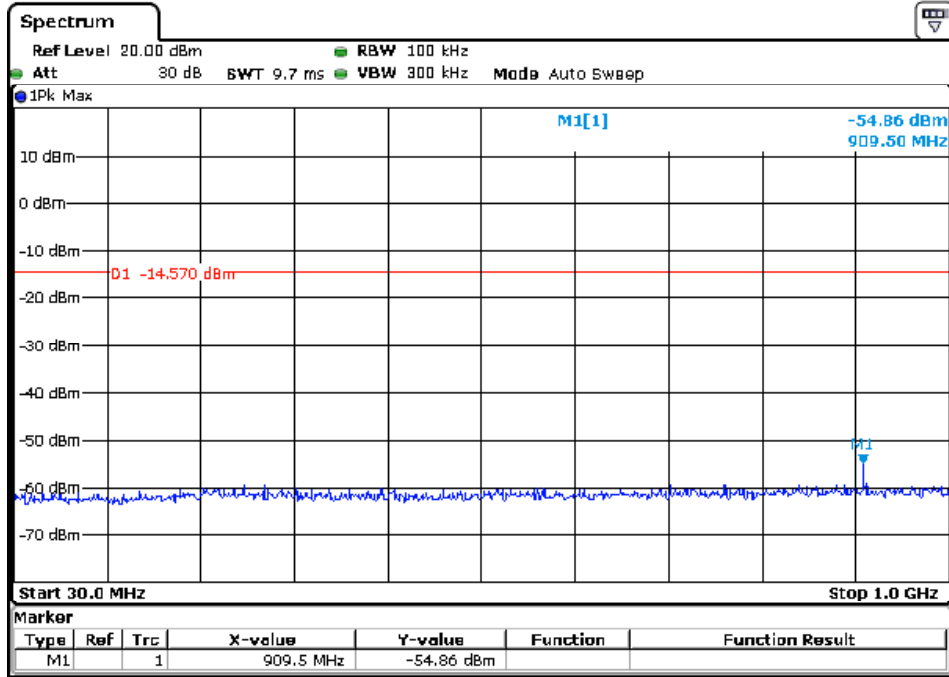
CH 1 (B mode) - Frequency Band 1 (30 MHz \leq f \leq 1000 MHz)
