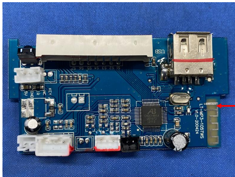
PCB Antenna
