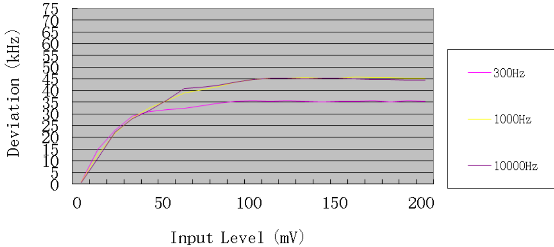
Modulation Limit
