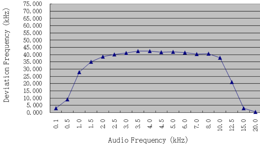
Frequency Response
