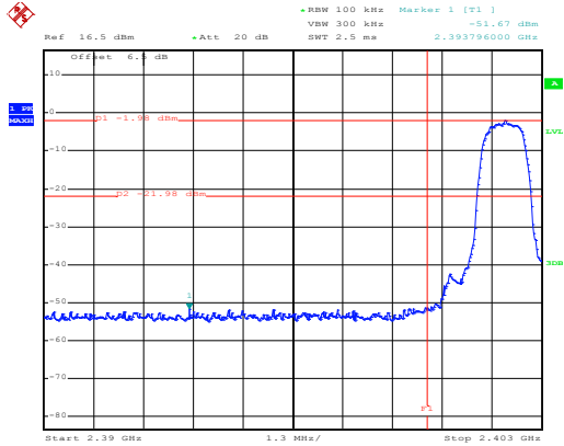
No-hopping mode
