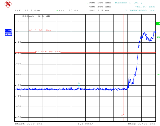
Hopping mode
