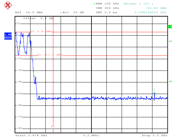
Hopping mode
