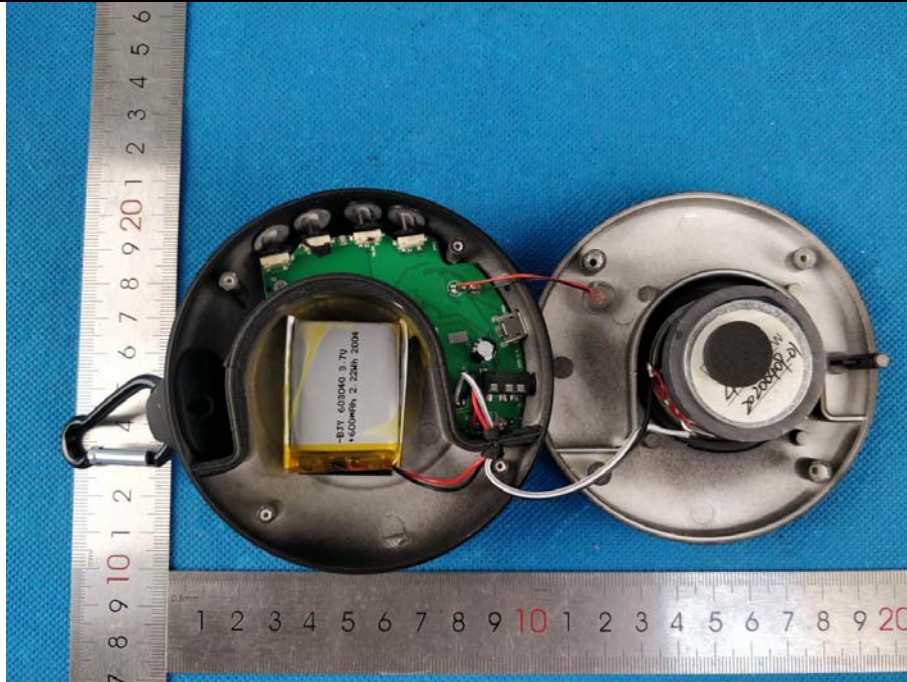
Photo 1 (For model SP-SA2BT)
