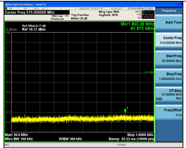
π/4-DQPSK on Channel 78
