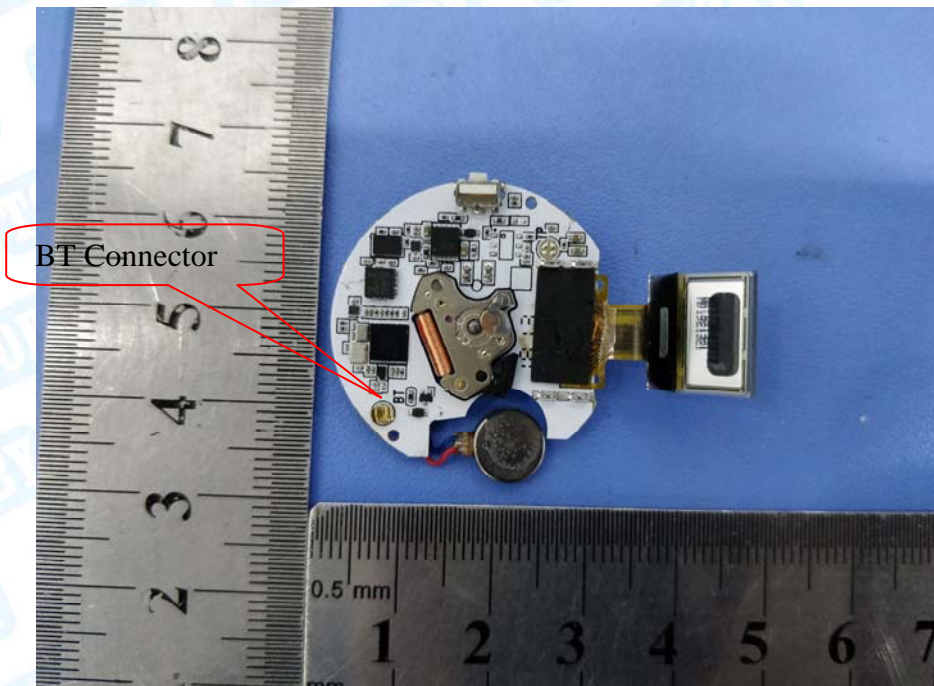
Photo 10 Appearance of PCB
