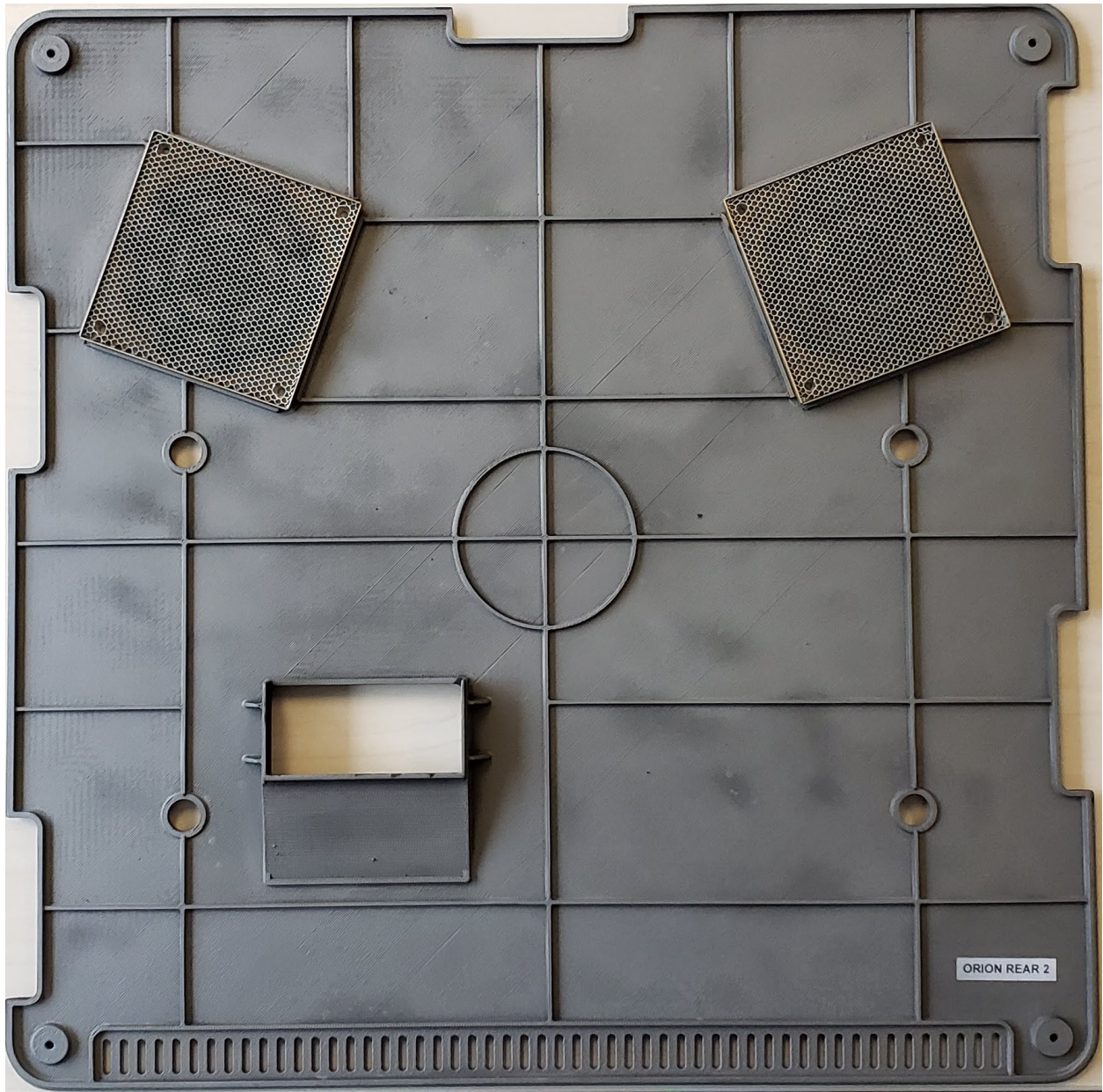
Figure 4: CotaTx203 Power Source, Rear Enclosure Interior
