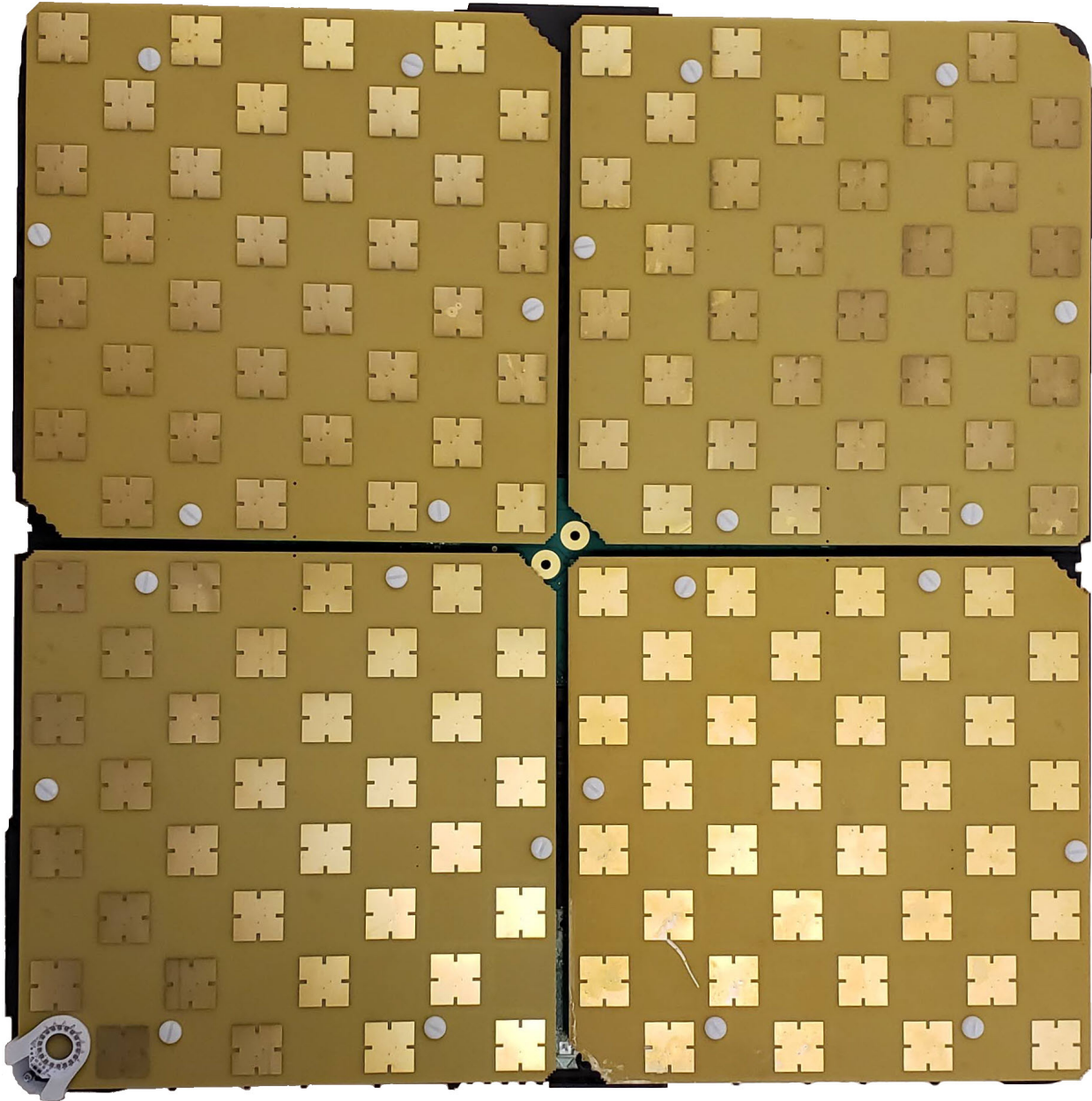
Figure 2: CotaTx203 Power Source, Frame Interior, Antenna-Side
