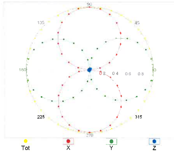
f=1800 MHz,R22,0°
