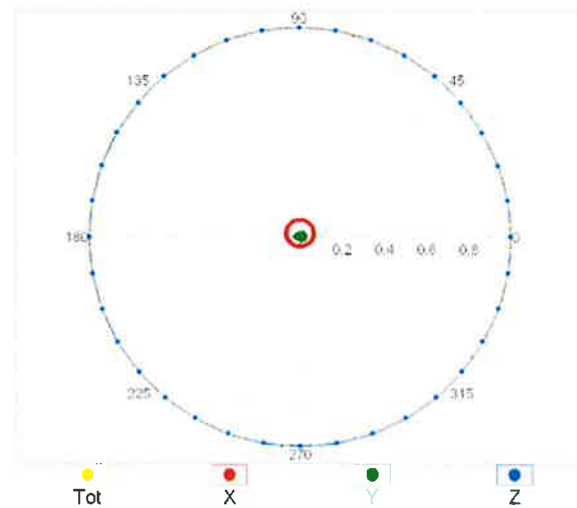
f=1800 MHz,R22,90°
