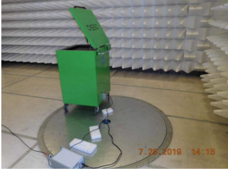
Test setup
