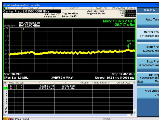
3MHz/16QAM/High CH
