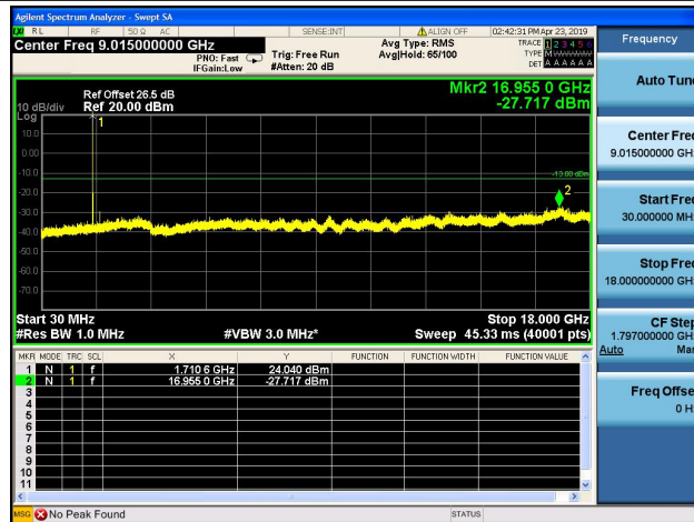
3MHz/16QAM/Mid CH
