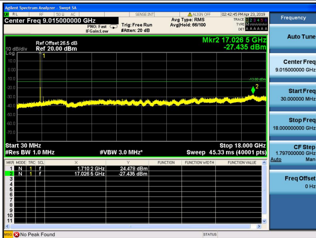
3MHz/QPSK/Mid CH
