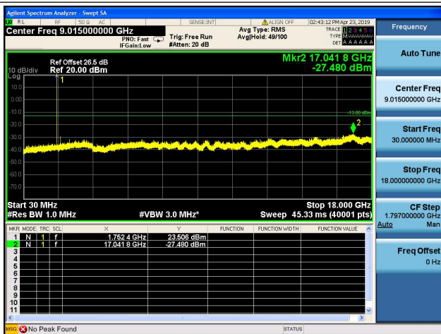
3MHz/QPSK/High CH
