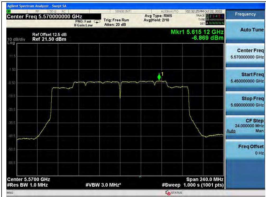
(Channel 114, 5570MHz, 802.11ax (HEW160), ANT0)
