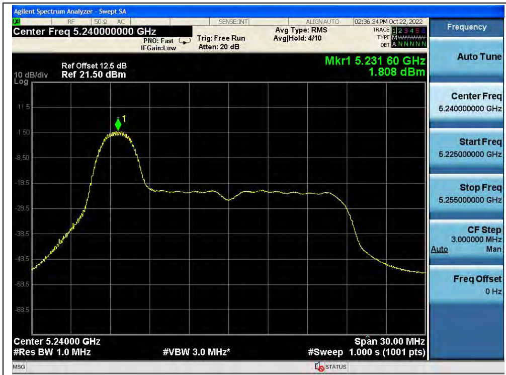
(Channel 48, 5240MHz, 802.11ax (HEW20) RU26, ANT0)
