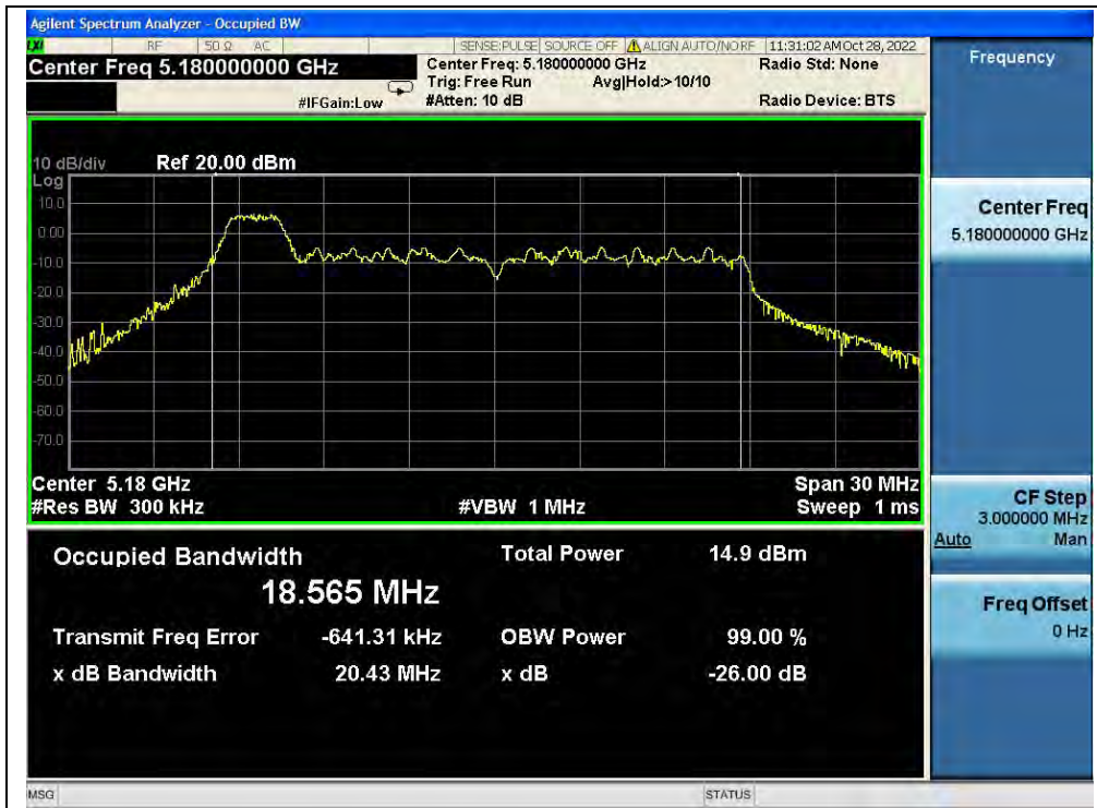
(Channel 36, 5180MHz, 802.11ax (HEW20) RU26)
