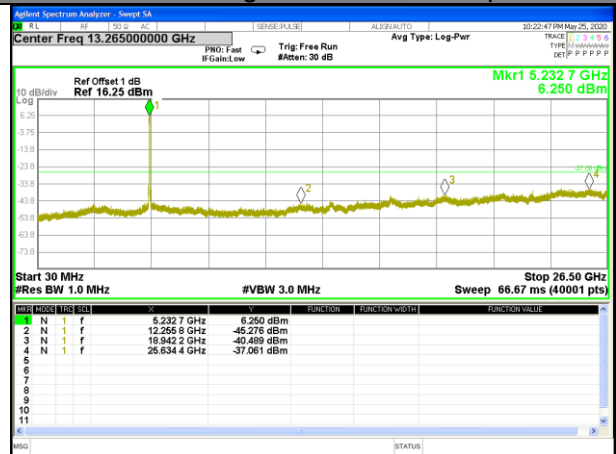
W52_11n40_Higher_Conducted Spurious
