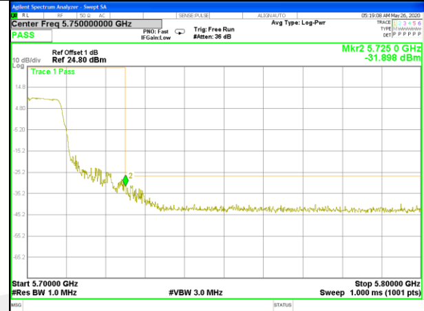
W56_11ac40_Middle_Conducted Spurious
