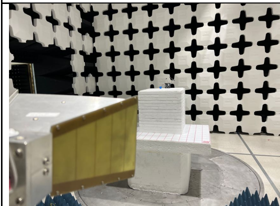
RE Test Above 1GHz Front View
