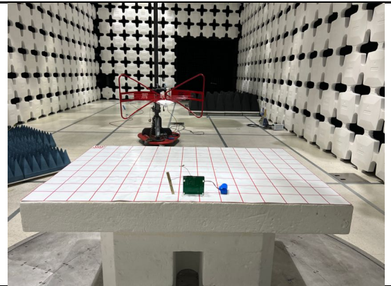
RE Test below 1GHz Rear View
