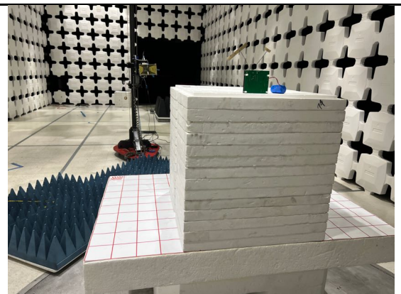
RE Test Above 1GHz Rear View
