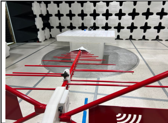
RE Test below 1GHz Front View
