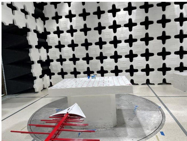
RE Below 1GHz – Front View
