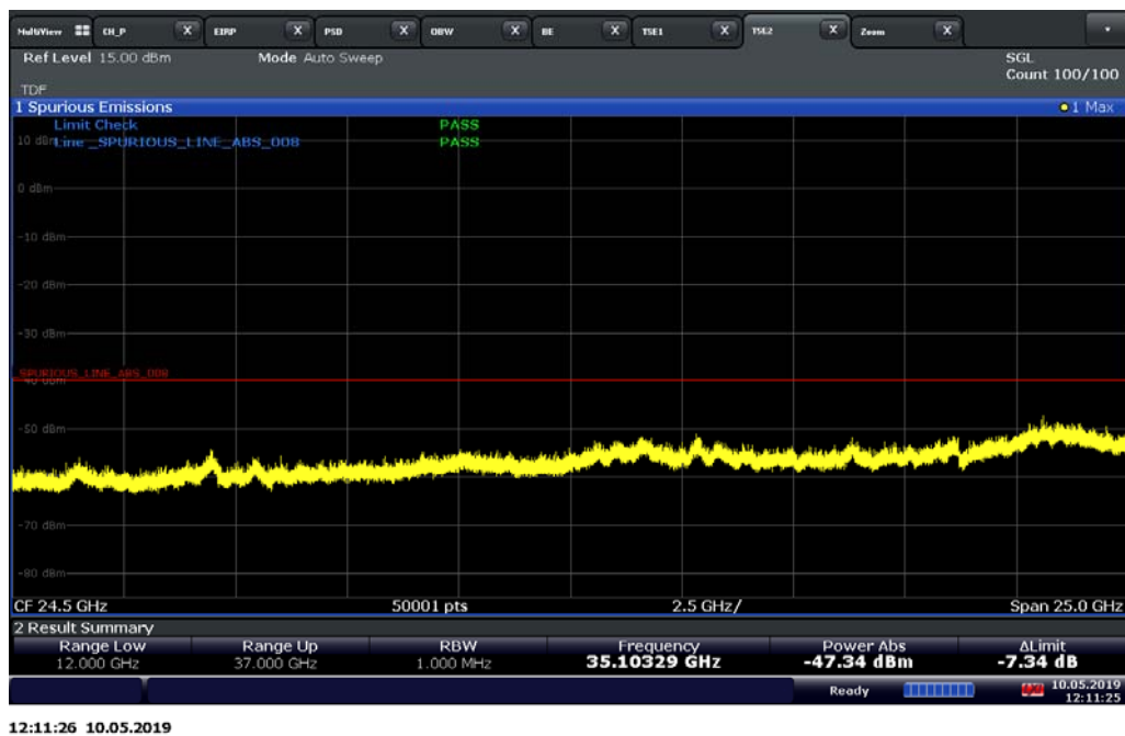
LTE Band 48 / 10 MHz / 64QAM – Low Channel_2
