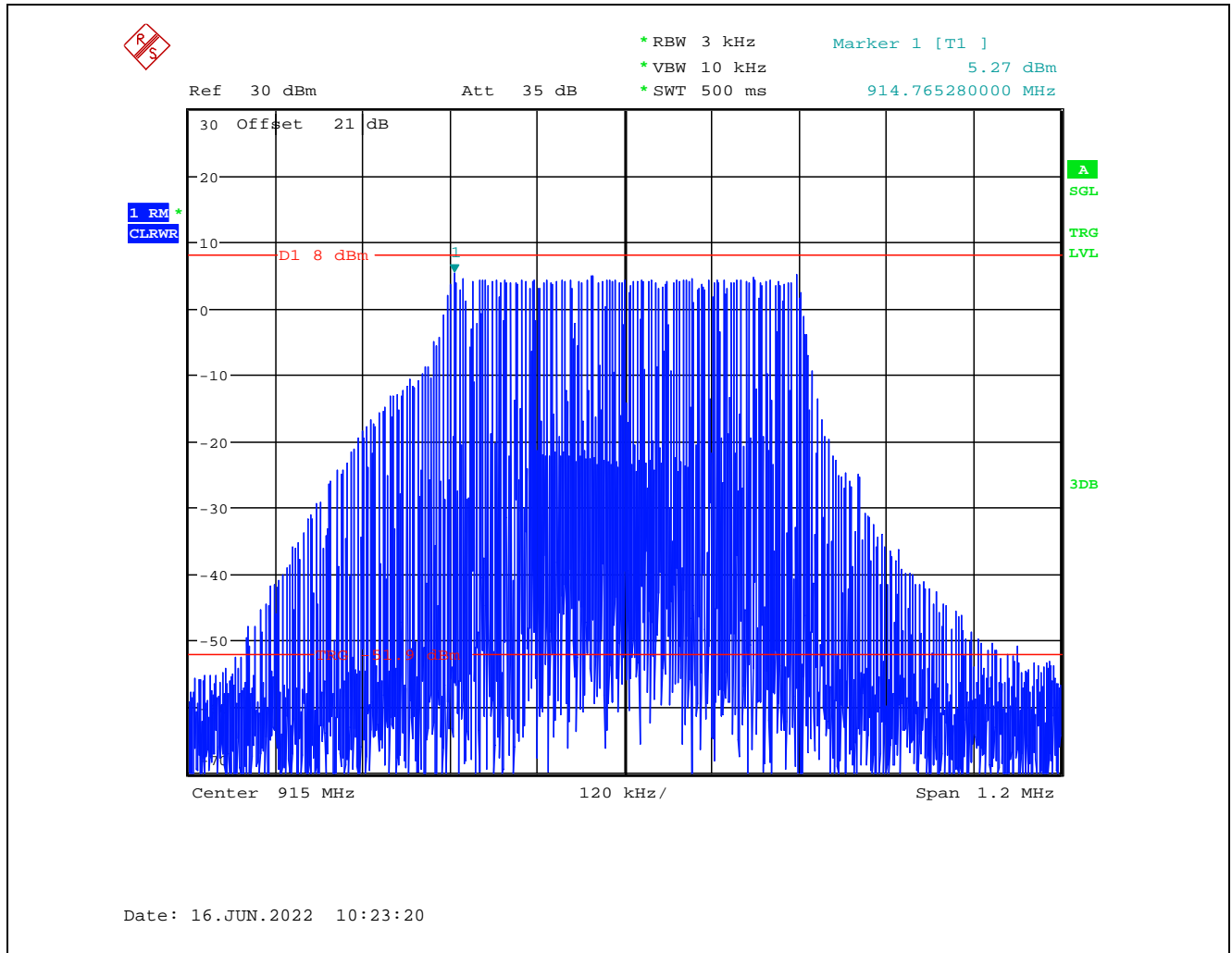
Plot 5.4.4.1. Power Spectral Density, LoRa Modulation, 915 MHz Sweep points: 5000, Sweep time: 500ms, Single sweep, Auto sweep time: 135ms
