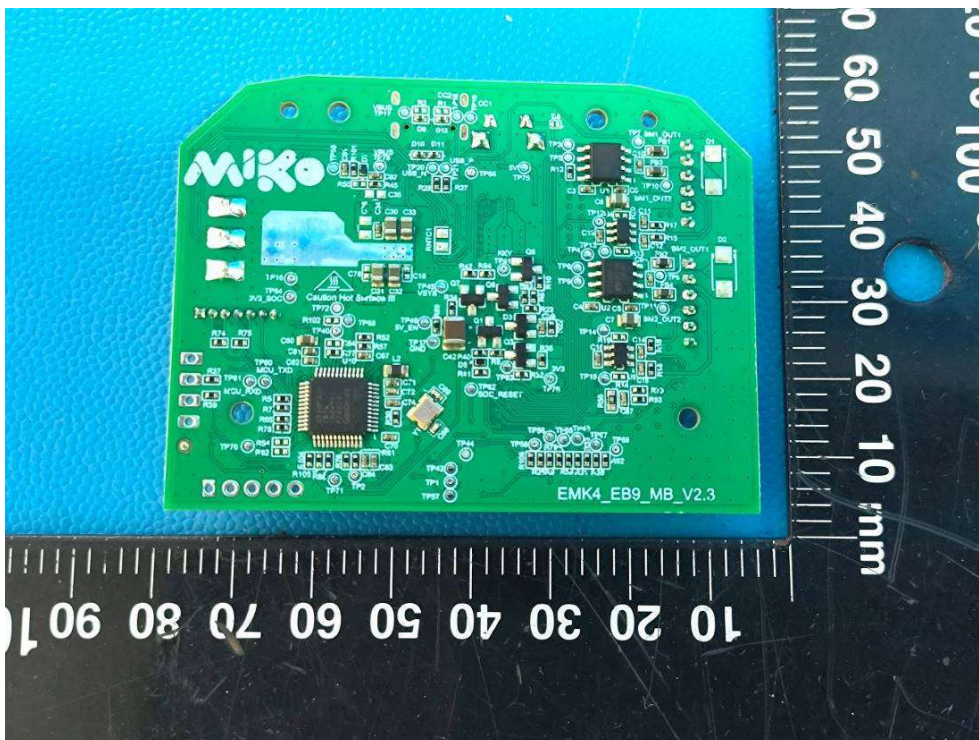
PCB view
