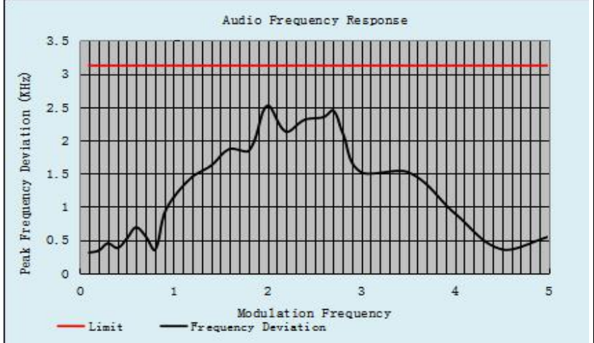
Channel 1: 462.5625MHz
