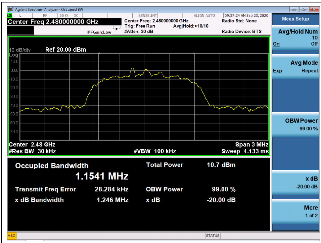
(Channel 78, 8-DPSK)
