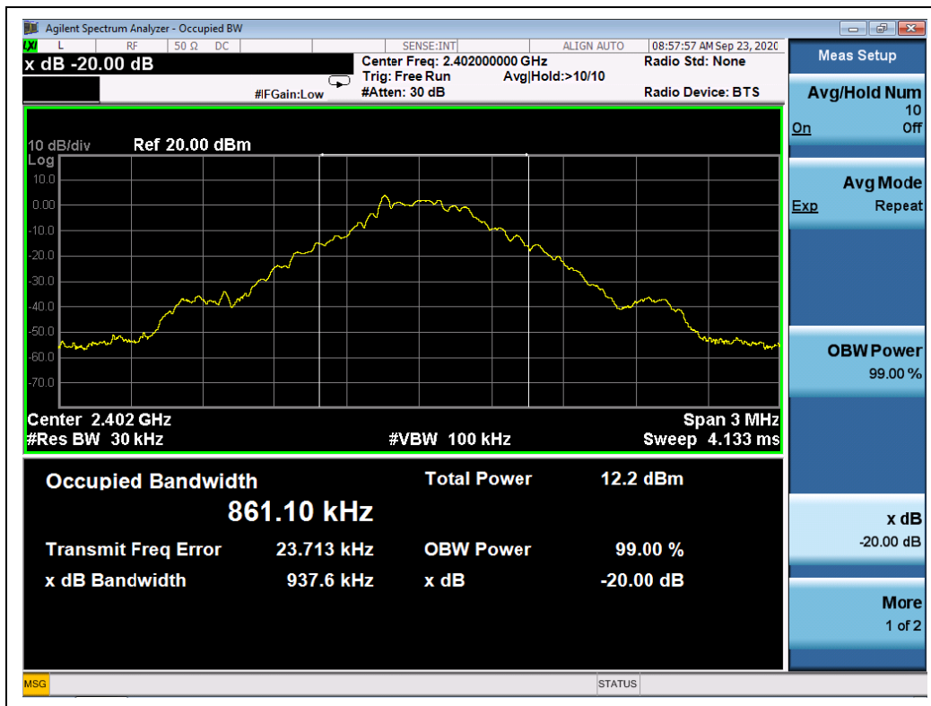
(Channel 0, GFSK)
