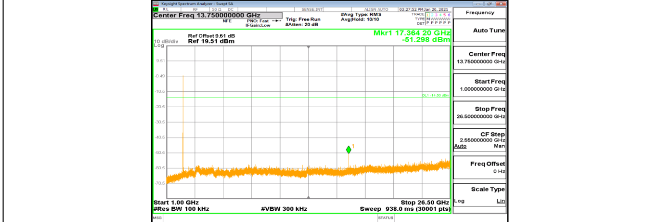
ZIGBEE_Ant1_2480_1000~26500
