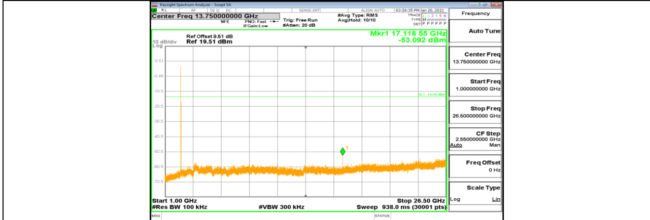
ZIGBEE_Ant1_2445_1000~26500
