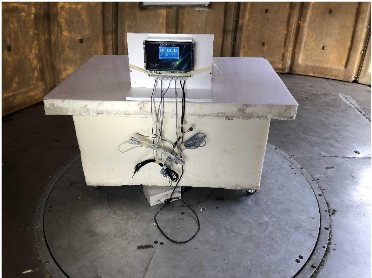
Test setup on OATS (worth case)
