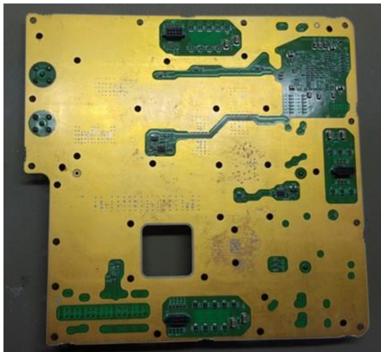
Figure 4: RF Board (Bottom)
