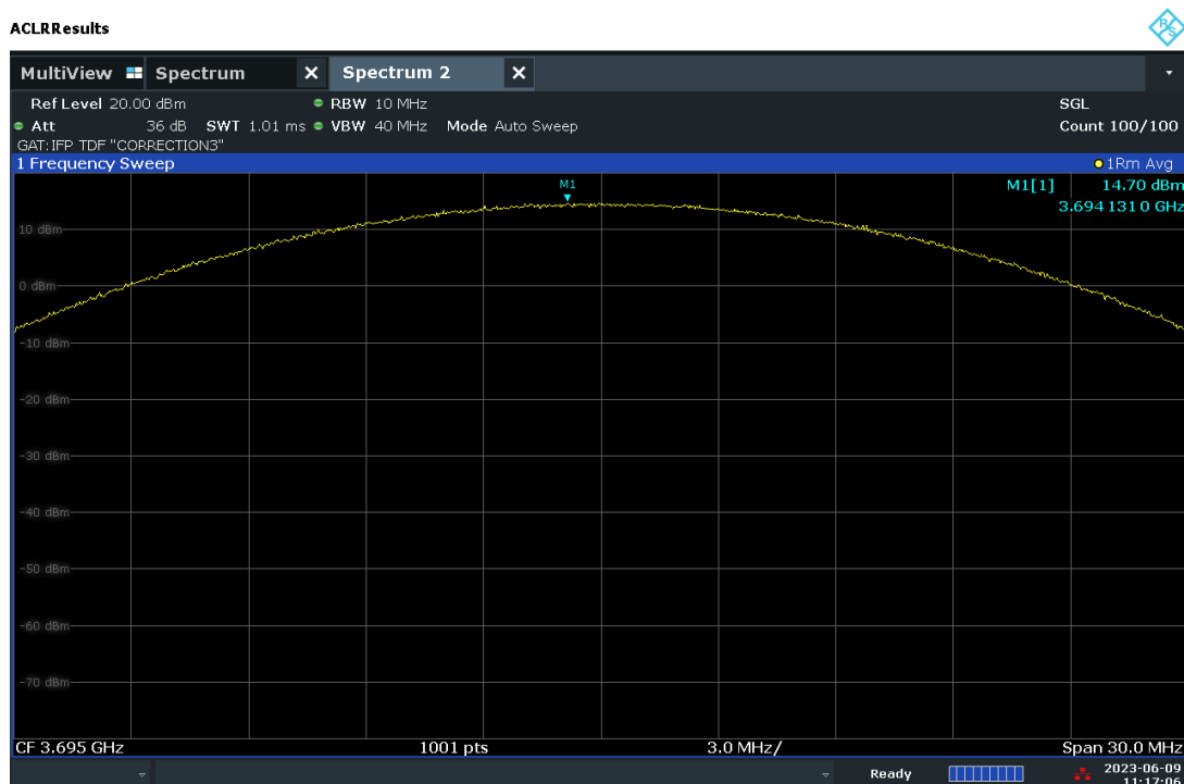
Plot 7.34. Conducted Power / 10MHz Plot (10MHz 16QAM, High Channel – Ch.A)
