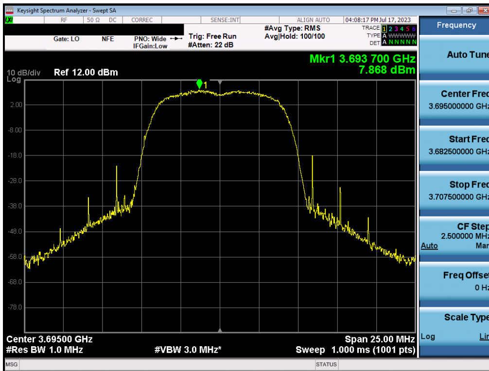
Plot 7.66. Conducted Power Spectral Density Plot (10MHz 16QAM, High Channel – Ch.A)
