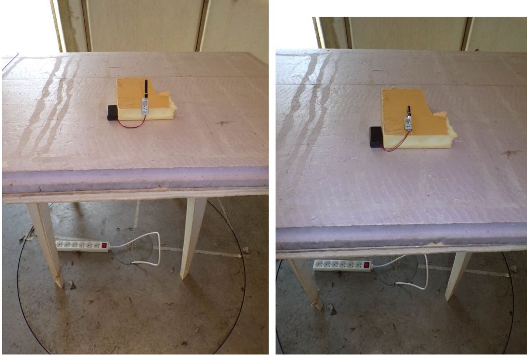
Measurements below 1GHz (Open Area Test Site)
