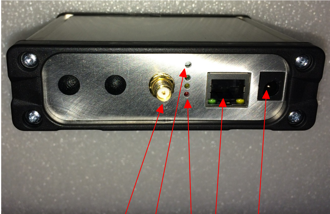
915 MHz antenna Hardware Reset LED indicator Ethernet connector 12V Power input
