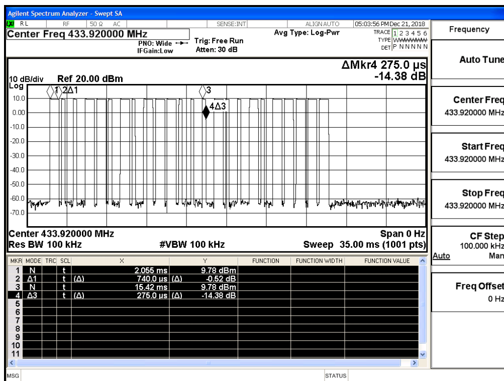
Pulse width
