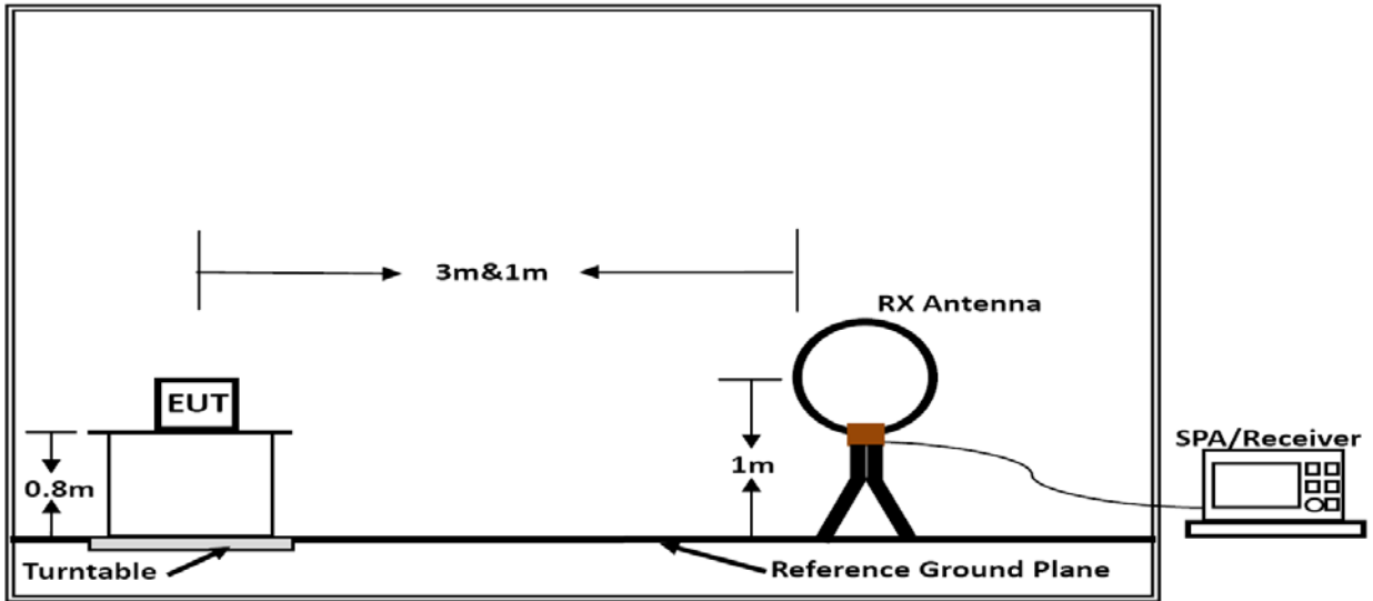
Below 30MHz
