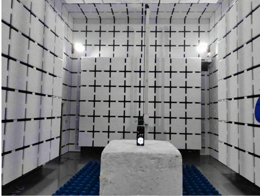
Radiated Emissions
