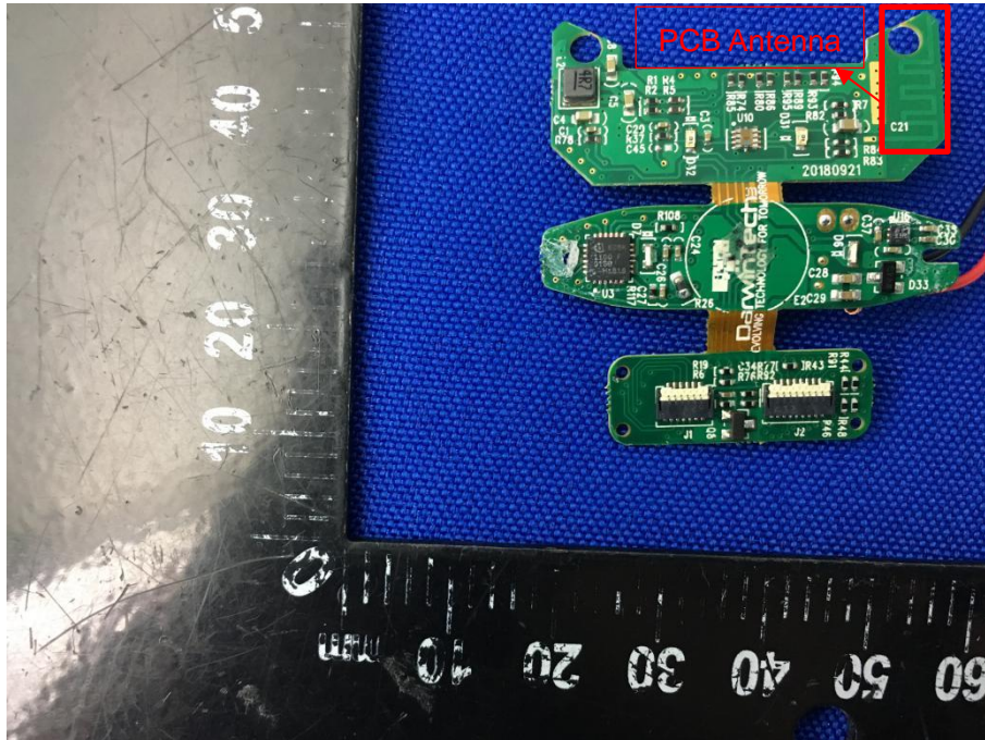
MAIN BOARD TOP VIEW (Mouth)
