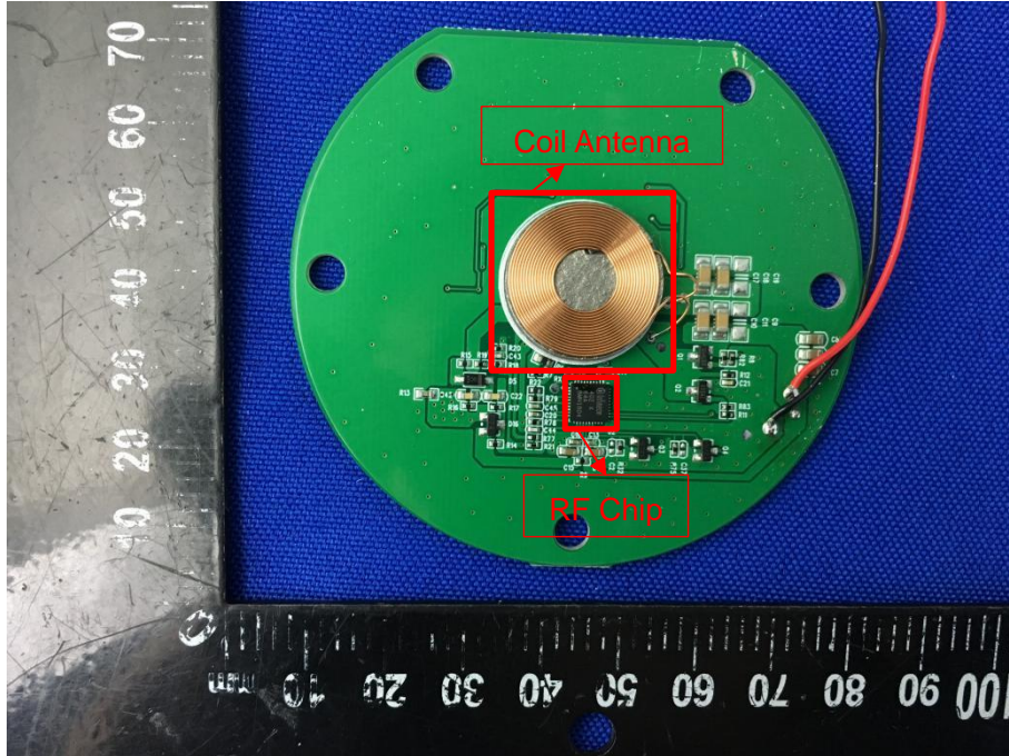
MAIN BOARD TOP VIEW (Cradle)
