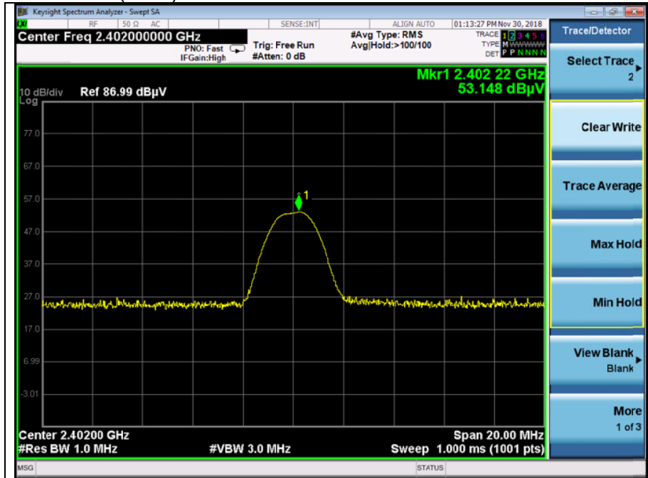
Low channel fundamental (Peak)
