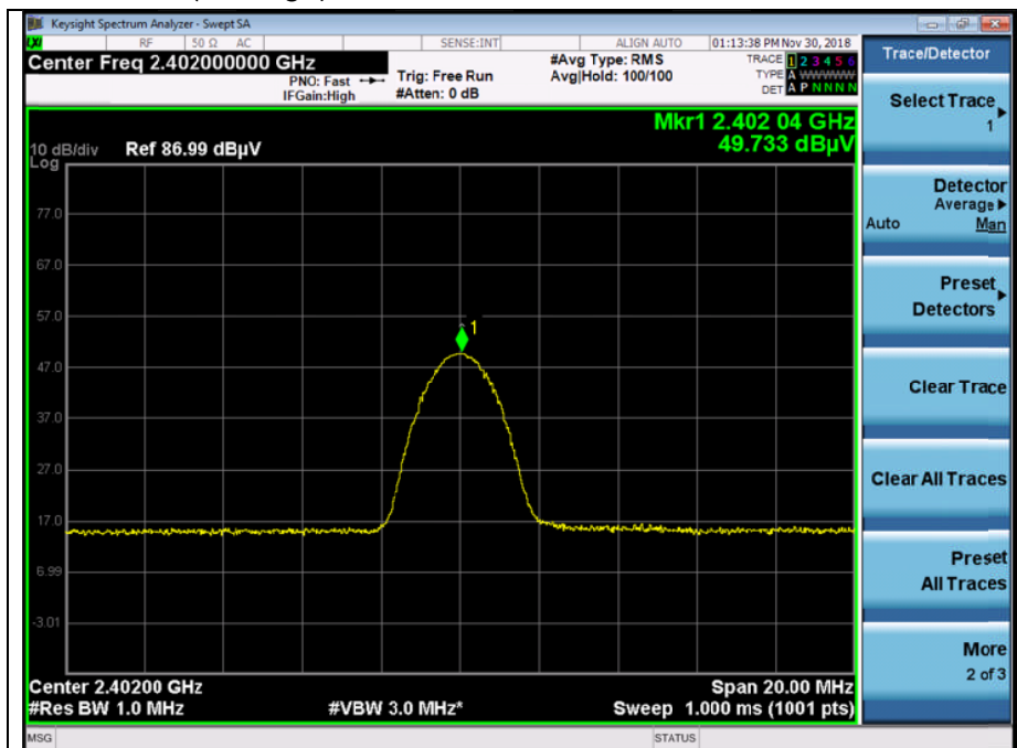
Low channel fundamental (Average)
