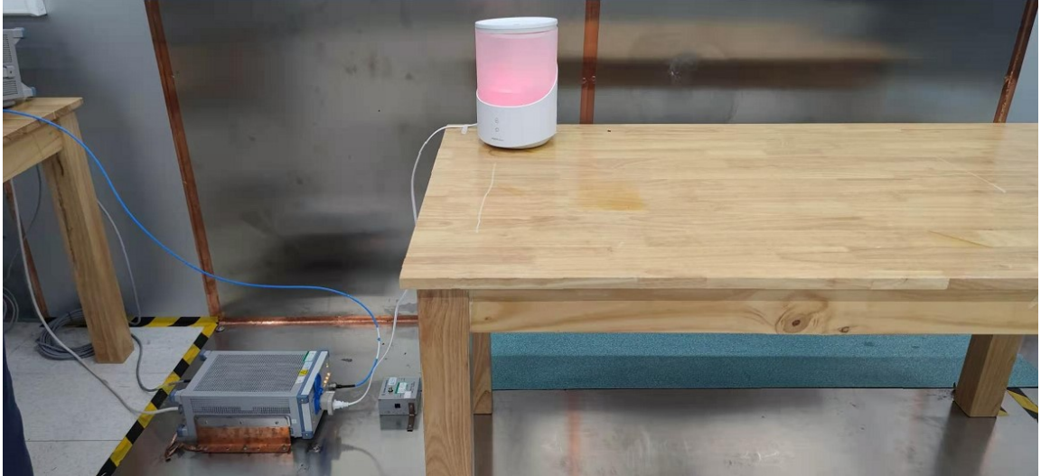
Photograph 3: Set-up photo for AC Conducted Emission
