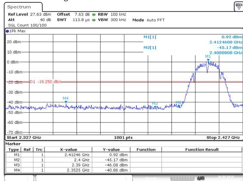
Band Edge NVNT 802.11b 2412MHz Ant1 Emission
