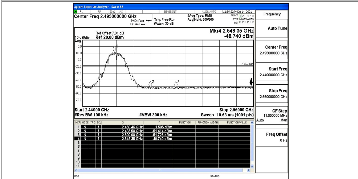
11B_Ant1_High_2462
