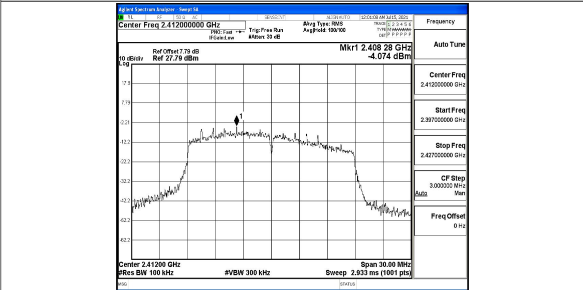
11N20SISO_Ant1_2412_0~Reference
