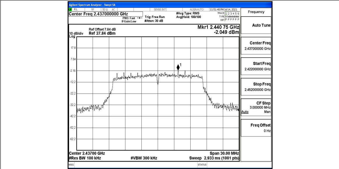
11G_Ant1_2437_0~Reference
