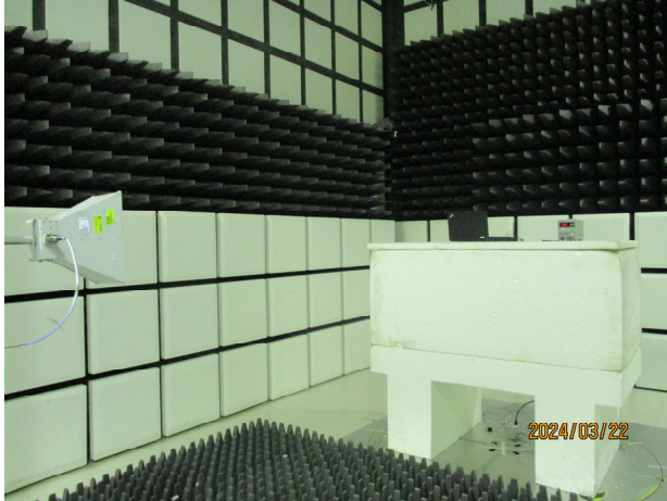
Part_15_247_LE_Radiated_Internal Antenna_Setup
