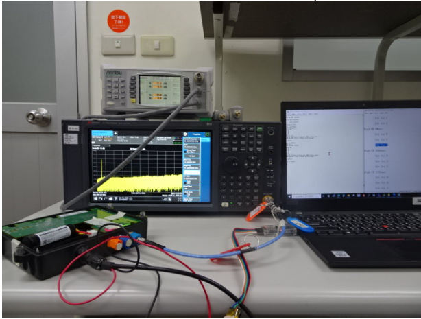
Part_15_247_LE_Radiated_Internal Antenna_Setup
