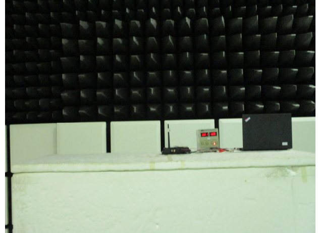
Part_15_247_LE_Radiated_External Antenna_Setup
