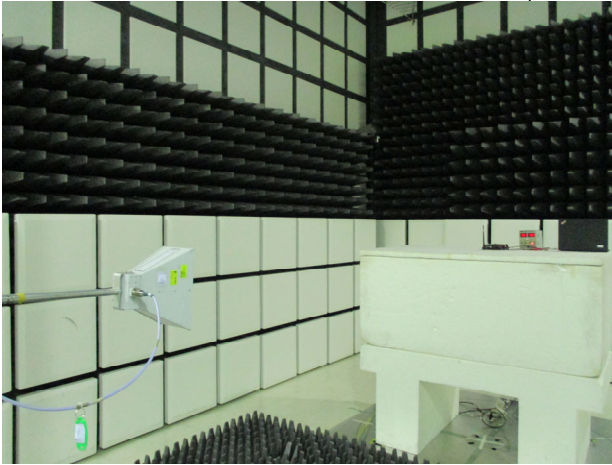
Part_15_247_LE_Radiated_External Antenna_Setup
