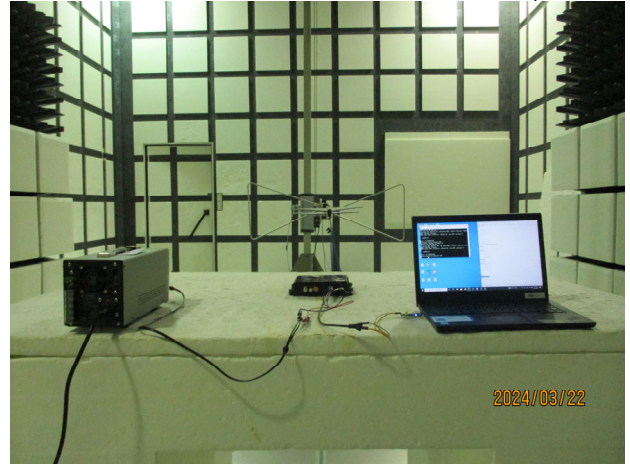
Part_15_247_LE_Radiated_Internal Antenna_Setup
