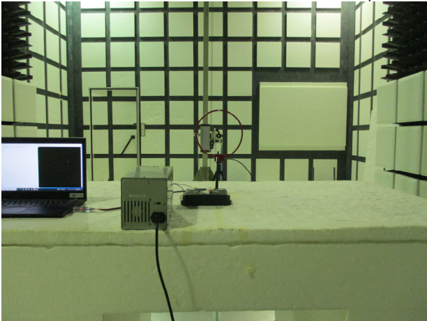
Part_15_247_LE_Radiated_External Antenna_Setup
