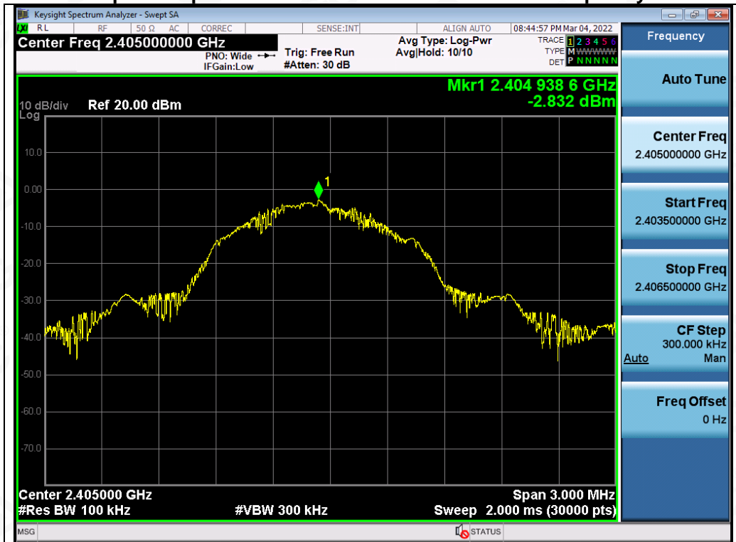
Test_Graph_GFSK_ANT1_2405_Reference Level
