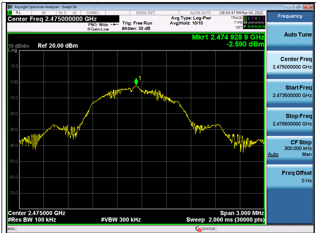
Test_Graph_GFSK_ANT1_2475_Reference Level
