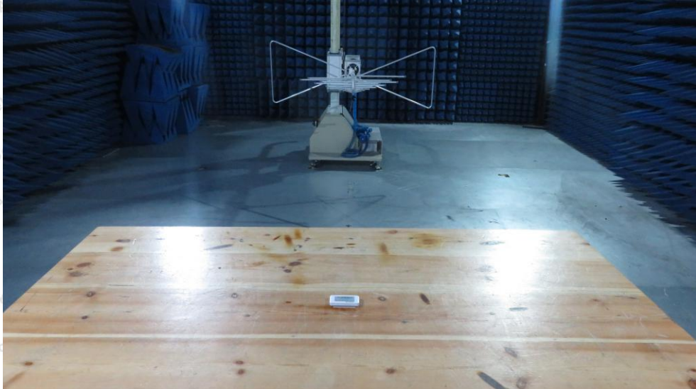
Photo of Radiation Emission Test
