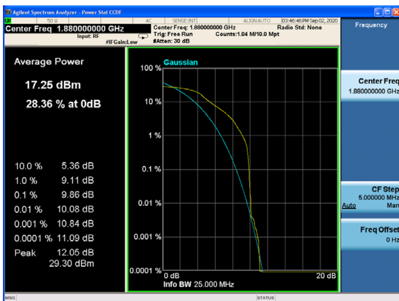
Peak-Average Ratio Plot(20MHz BW,QPSK,Band 2-mid Channel)
