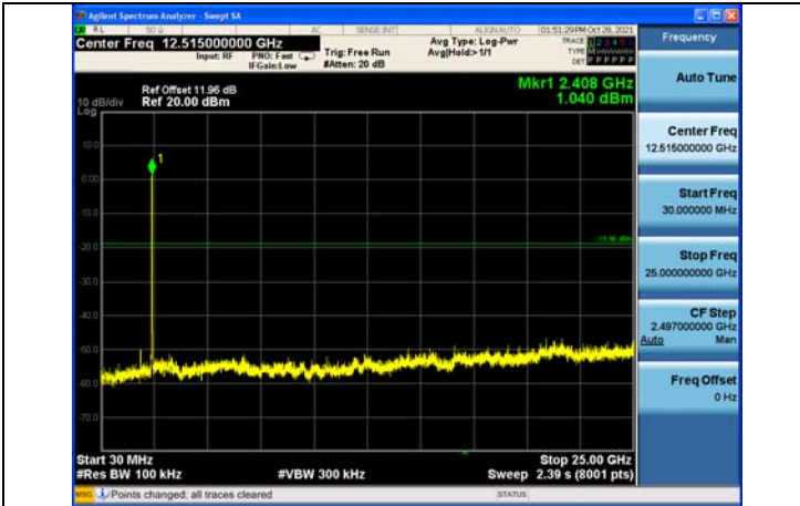
Test Mode:802.11n HT20 2412MHz Chain0
