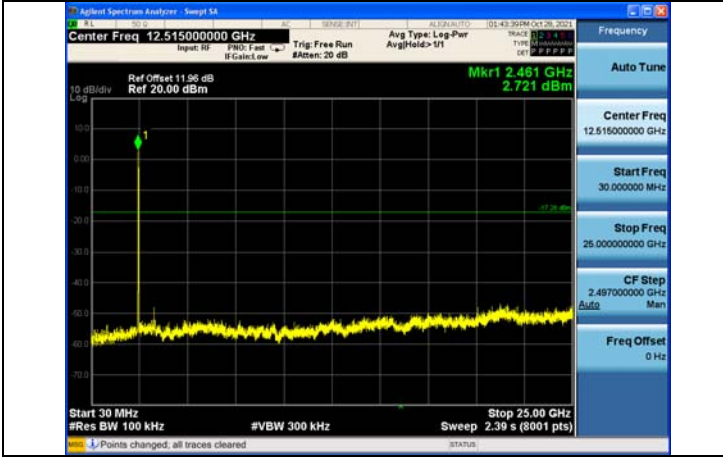
Test Mode:802.11g 2462MHz Chain0
