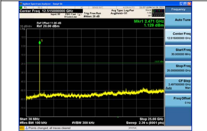
Test Mode:802.11n HT20 2462MHz Chain0
