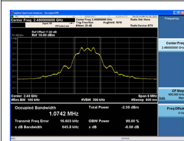
Modulation: Coded 125K 2480MHz
