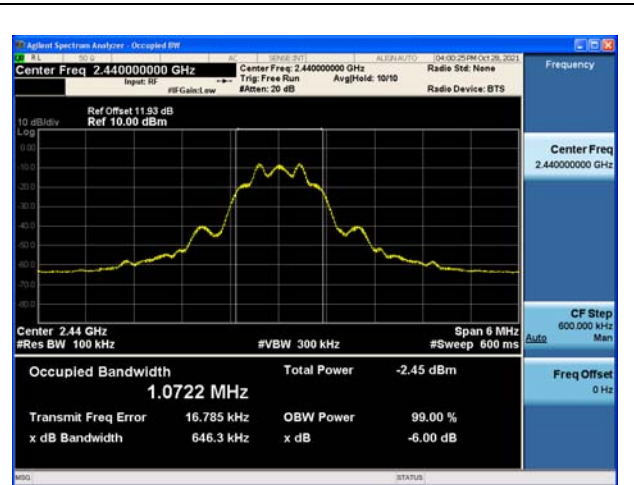
Modulation: Coded 125K 2440MHz
