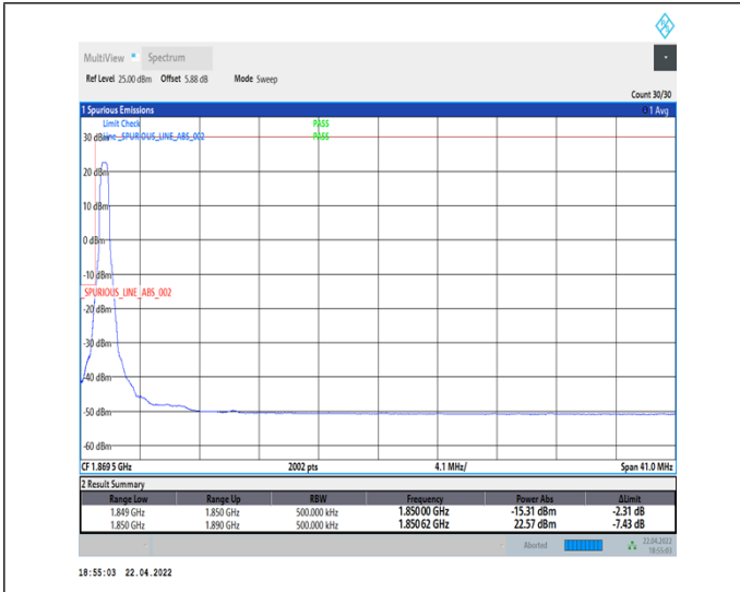
1-N25--15-40-L-1-DFT-PI2BPSK-Edge_1RB_Left-1@0-Ant1-seegraph-PASS-see graph
