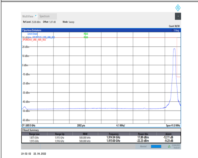
1-N25--15-40-H-5-CP-QPSK-Edge_1RB_Right-1@215-Ant1-seegraph-PASS-see graph
