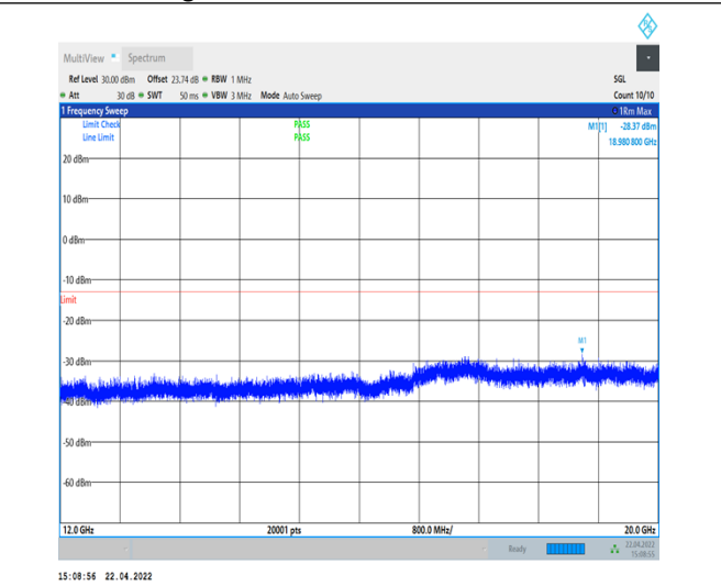
1-N25--15-40-H-1-DFT-PI2BPSK-Inner_1RB_Left- 1@1-12000-20000-Ant1--28.37--13-PASS
