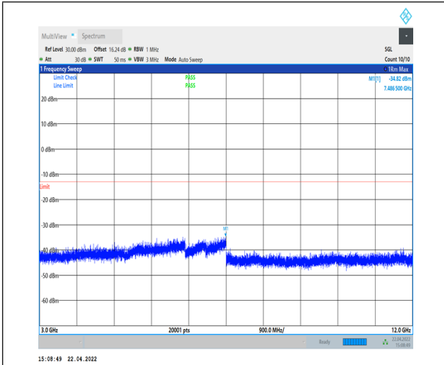
1-N25--15-40-H-1-DFT-PI2BPSK-Inner_1RB_Left- 1@1-3000-12000-Ant1--34.82--13-PASS
