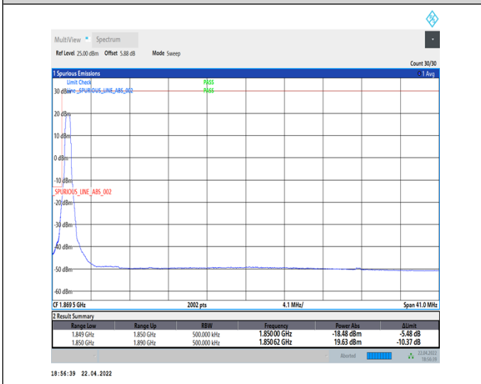
1-N25--15-40-L-4-CP-QPSK-Edge_1RB_Left-1@0-Ant1-seegraph-PASS-see graph
