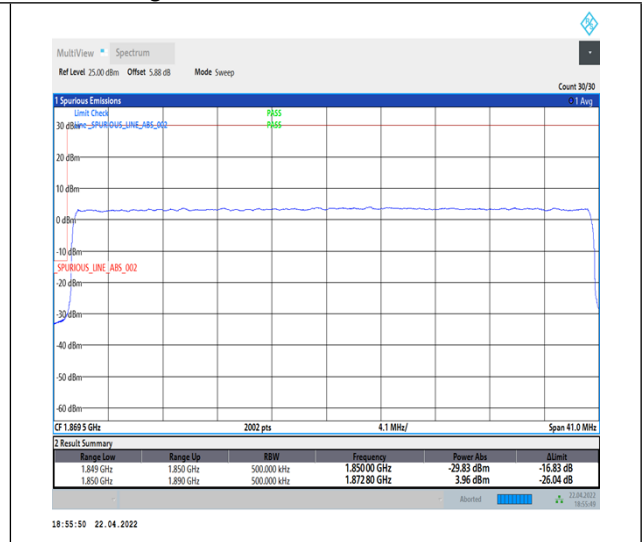
1-N25--15-40-L-3-DFT-PI2BPSK-Outer_Full-216@0-Ant1-seegraph-PASS-see graph
