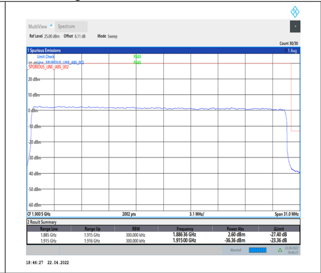
1-N25--15-30-H-3-DFT-PI2BPSK-Outer_Full-160@0-Ant1-seegraph-PASS-see graph
