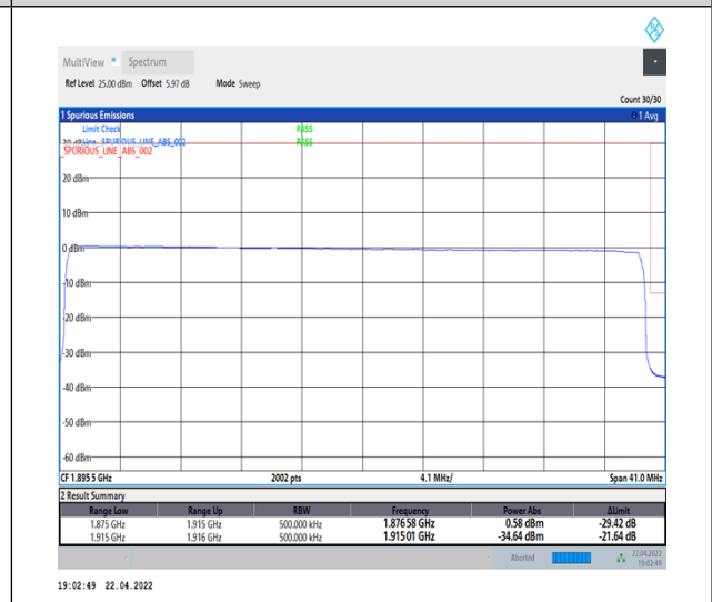
1-N25--15-40-H-6-CP-QPSK-Outer_Full-216@0-Ant1-seegraph-PASS-see graph
