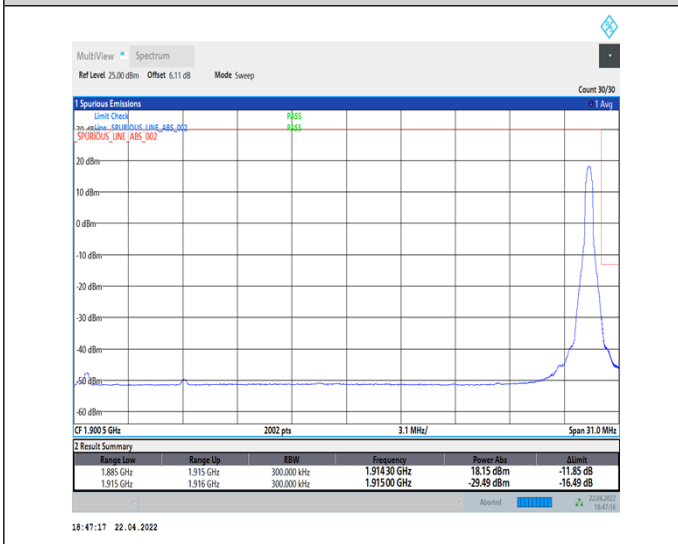
1-N25--15-30-H-5-CP-QPSK-Edge_1RB_Right-1@159-Ant1-seegraph-PASS-see graph
