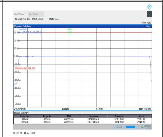
1-N25--15-40-L-6-CP-QPSK-Outer_Full-216@0-Ant1-seegraph-PASS-see graph
