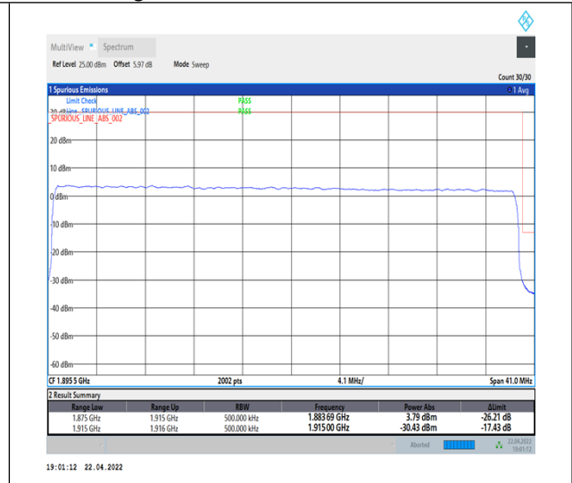
1-N25--15-40-H-3-DFT-PI2BPSK-Outer_Full-216@0-Ant1-seegraph-PASS-see graph
