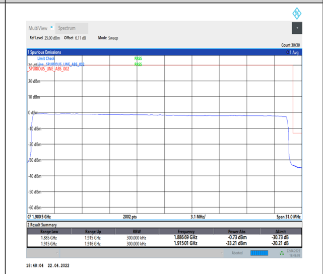
1-N25--15-30-H-6-CP-QPSK-Outer_Full-160@0-Ant1-seegraph-PASS-see graph
