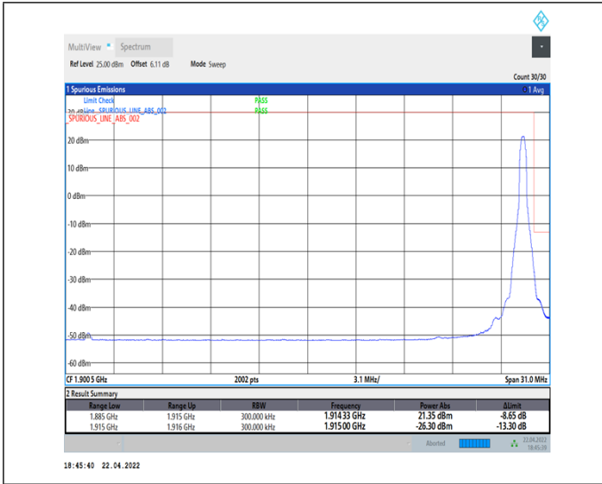
1-N25--15-30-H-2-DFT-PI2BPSK-Edge_1RB_Right-1@159-Ant1-seegraph-PASS-see graph
