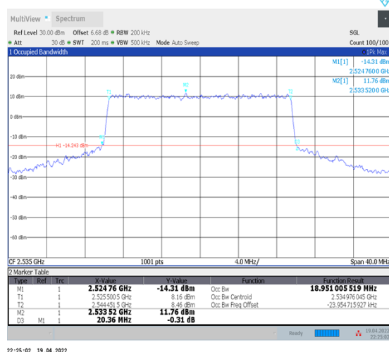
1-N7--15-20-M-6-CP-QPSK-Outer_Full-106@0- Ant1-18.951-20.360-≤20-PASS
