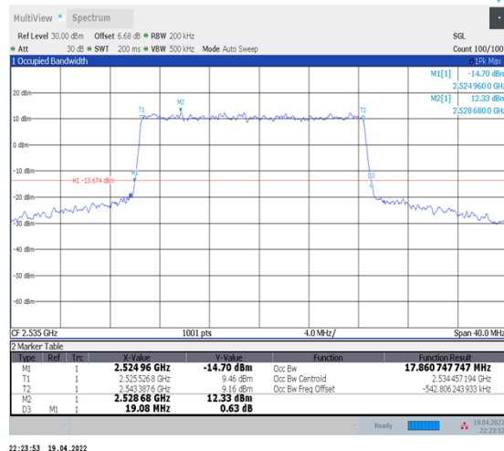
1-N7--15-20-M-4-DFT-64QAM-Outer_Full-100@0- Ant1-17.861-19.080-≤20-PASS
