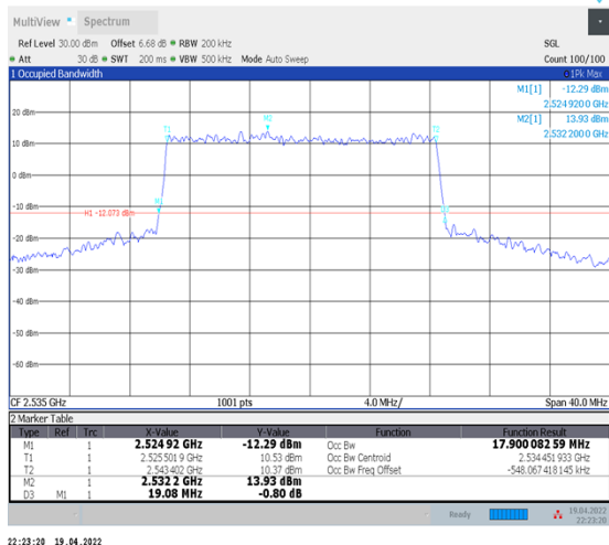
1-N7--15-20-M-3-DFT-16QAM-Outer_Full-100@0- Ant1-17.9-19.080-≤20-PASS
