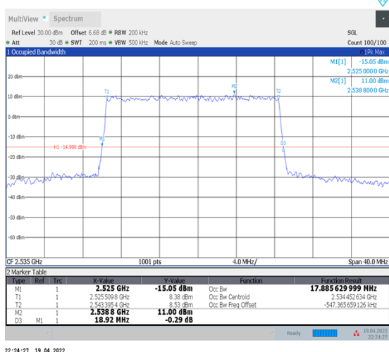
1-N7--15-20-M-5-DFT-256QAM-Outer_Full-100@0- Ant1-17.886-18.920-≤20-PASS
