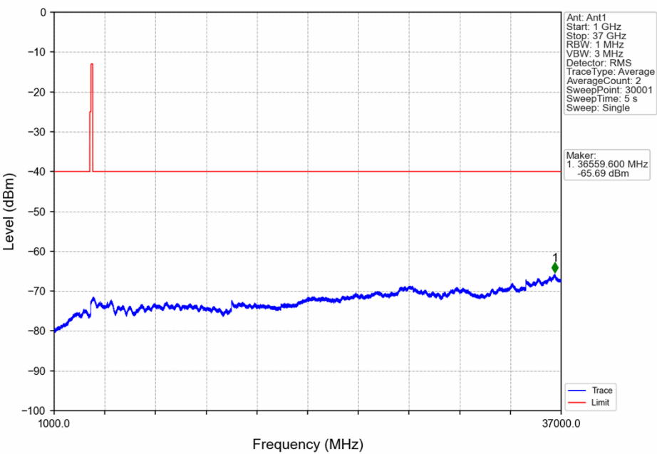
n48_30kHz_SISO_NTNV_40MHz_DFT-s-OFDM QPSK_3679.98MHz_Outer_Full
