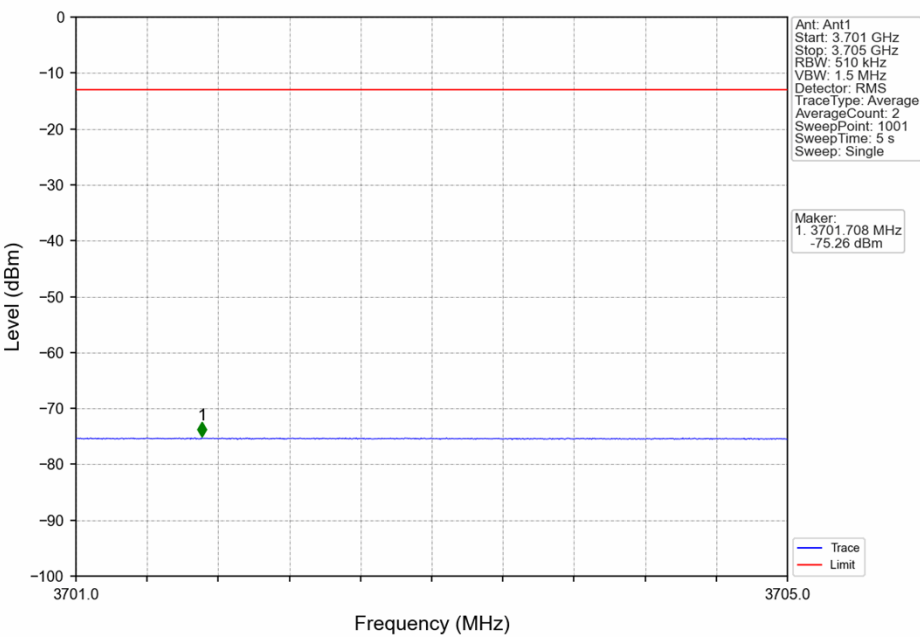
n48_30kHz_SISO_NTNV_40MHz_DFT-s-OFDM QPSK_3679.98MHz_Outer_Full
