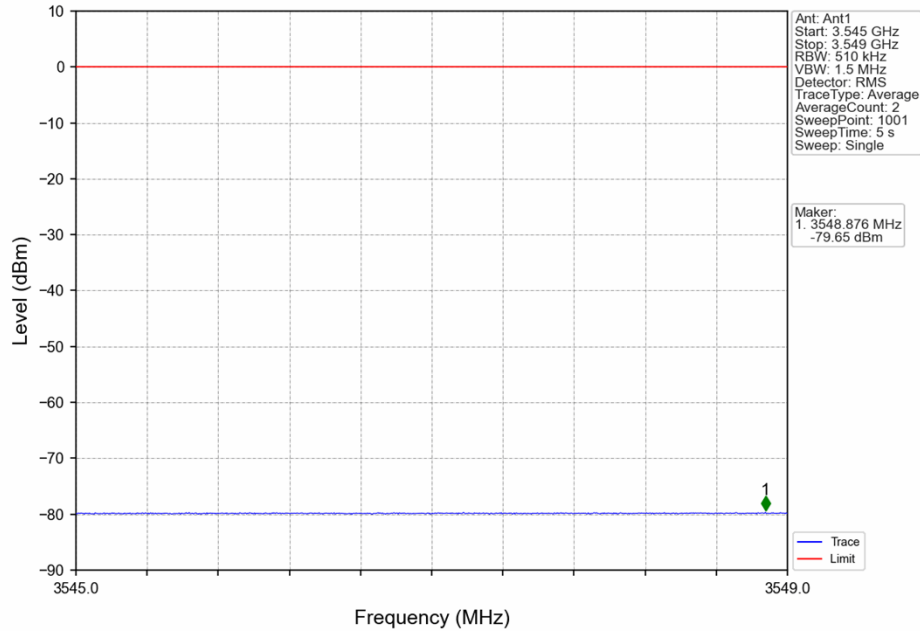
n48_30kHz_SISO_NTNV_40MHz_CP-OFDM QPSK_3570MHz_Outer_Full
