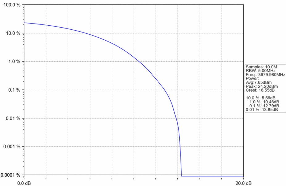
n48_30kHz_SISO_NTNV_40MHz_CP-OFDM QPSK_3679.98MHz_Outer_Full
