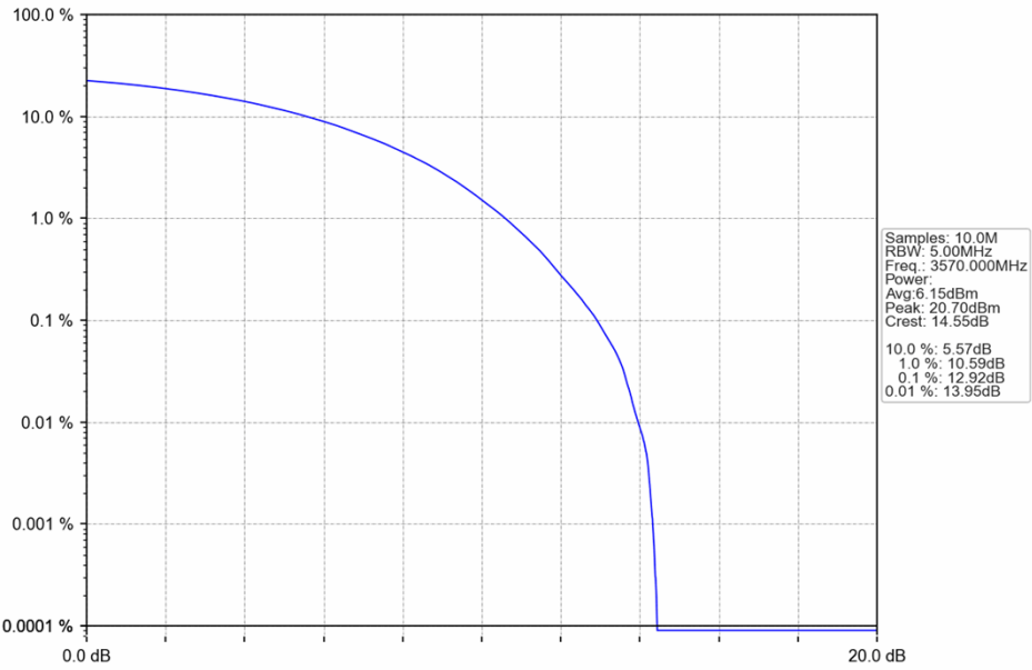
n48_30kHz_SISO_NTNV_40MHz_CP-OFDM QPSK_3570MHz_Outer_Full
