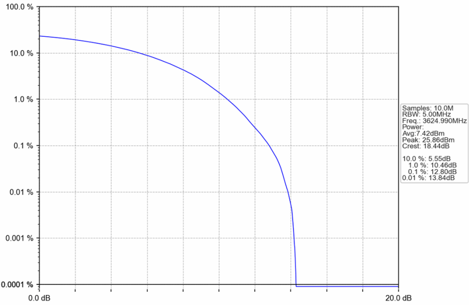
n48_30kHz_SISO_NTNV_40MHz_CP-OFDM QPSK_3624.99MHz_Outer_Full
