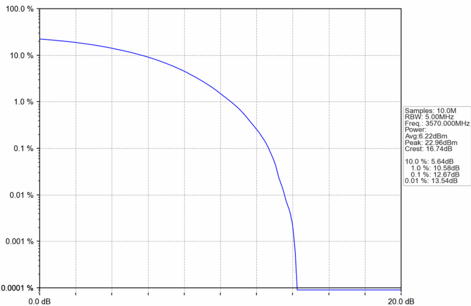
n48_30kHz_SISO_NTNV_40MHz_CP-OFDM 16 QAM_3570MHz_Outer_Full
