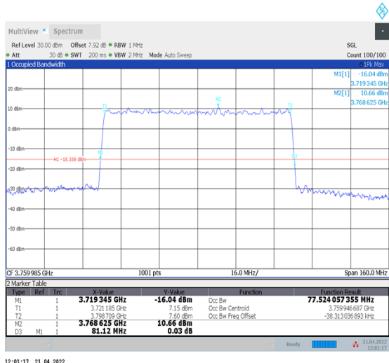
1-N78-3700-3800--30-80-H-9-CP-256QAM-Outer_Full-217@0-Ant1-77.524-81.120-≤80-PASS
