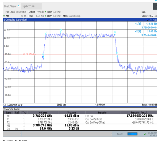
1-N78-3700-3800--30-20-H-2-DFT-PI2BPSK- Outer Full-50@0-Ant1-17.845-19.000-≤20-PASS
