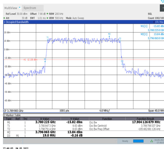
1-N78-3700-3800--30-20-H-4-DFT-64QAM- Outer Full-50@0-Ant1-17.904-19.000-≤20-PASS
