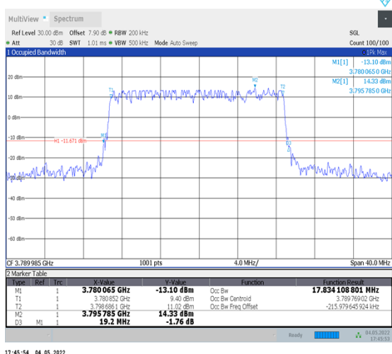
1-N78-3700-3800--30-20-H-3-DFT-16QAM- Outer Full-50@0-Ant1-17.834-19.200-≤20-PASS
