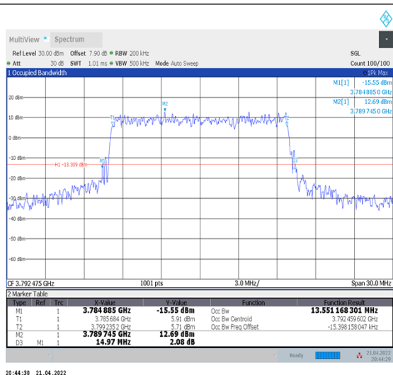
1-N78-3700-3800--30-15-H-8-CP-64QAM-Outer_Full-38@0-Ant1-13.551-14.970≤15-PASS
