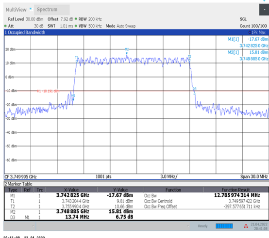
1-N78-3700-3800--30-15-M-1-DFT-QPSK-Outer_Full-36@0-Ant1-12.786-13.740≤15-PASS
