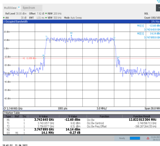
1-N78-3700-3800--30-15-M-4-DFT-64QAM-Outer_Full-36@0-Ant1-12.822-14.100≤15-PASS
