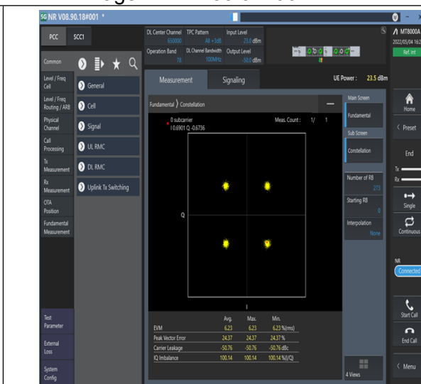
1-N78-3700-3800--30-100-M-6-CP-QPSK-Outer_Full-273@0-Ant1-see graph-PASS
