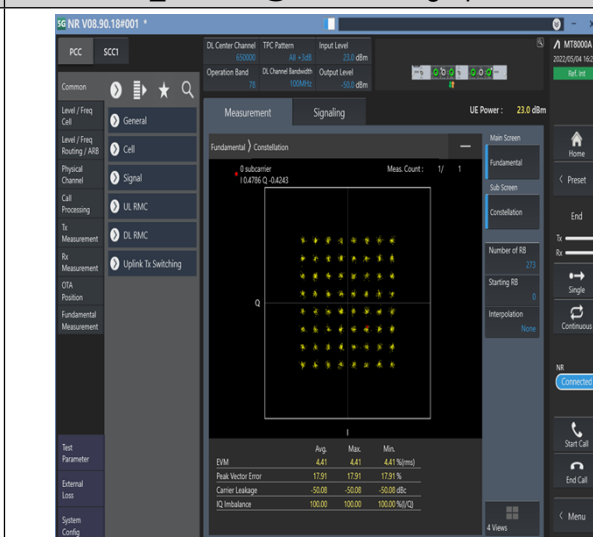
1-N78-3700-3800--30-100-M-8-CP-64QAM-Outer_Full-273@0-Ant1-see graph-PASS
