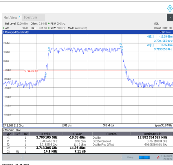
1-N78-3700-3800--30-15-L-2-DFT-PI2BPSK-Outer_Full-36@0-Ant1-12.883-14.100-≤15-PASS
