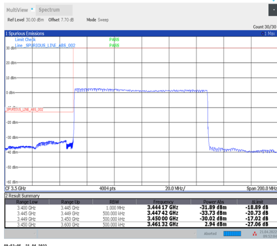
1-N78-3450-3550--30-100-L-3-DFT-PI2BPSK-Outer_Full-270@0-Ant1-PASS-see graph
