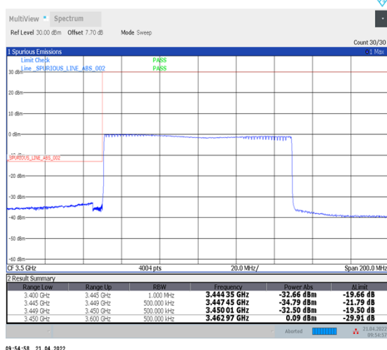
1-N78-3450-3550--30-100-L-6-CP-QPSK-Outer_Full-273@0-Ant1-PASS-see graph
