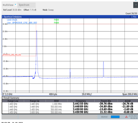
1-N78-3450-3550--30-100-L-1-DFT-PI2BPSK-Edge_1RB_Left-1@0-Ant1-PASS-see graph
