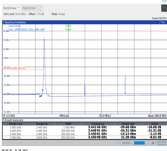
1-N78-3450-3550--30-100-L-4-CP-QPSK-Edge_1RB_Left-1@0-Ant1-PASS-see graph
