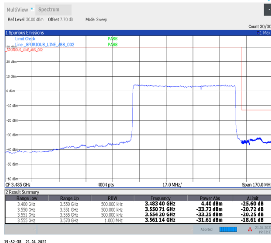
1-N78-3450-3550--30-70-H-3-DFT-PI2BPSK-Outer_Full-180@0-Ant1-PASS-see graph
