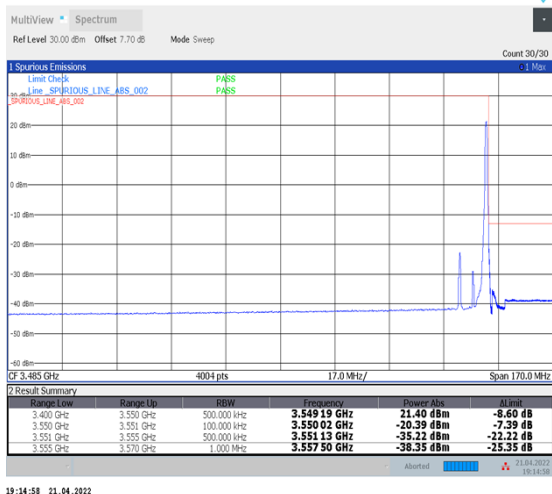
1-N78-3450-3550--30-10-H-2-DFT-PI2BPSK-Edge_1RB_Right-1@23-Ant1-PASS-see graph
