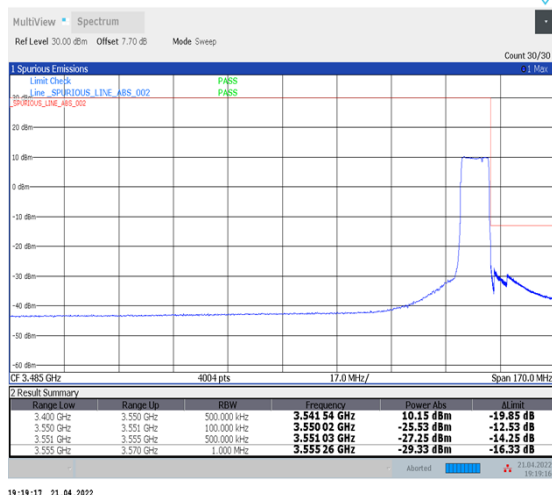
1-N78-3450-3550--30-10-H-6-CP-QPSK-Outer_Full-24@0-Ant1-PASS-see graph
