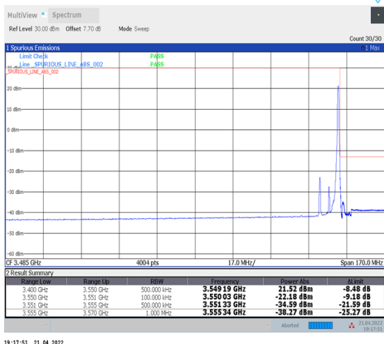
1-N78-3450-3550--30-10-H-5-CP-QPSK-Edge_1RB_Right-1@23-Ant1-PASS-see graph
