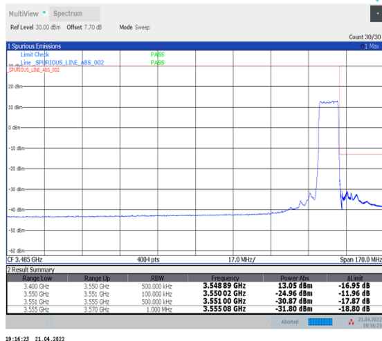
1-N78-3450-3550--30-10-H-3-DFT-PI2BPSK-Outer_Full-24@0-Ant1-PASS-see graph
