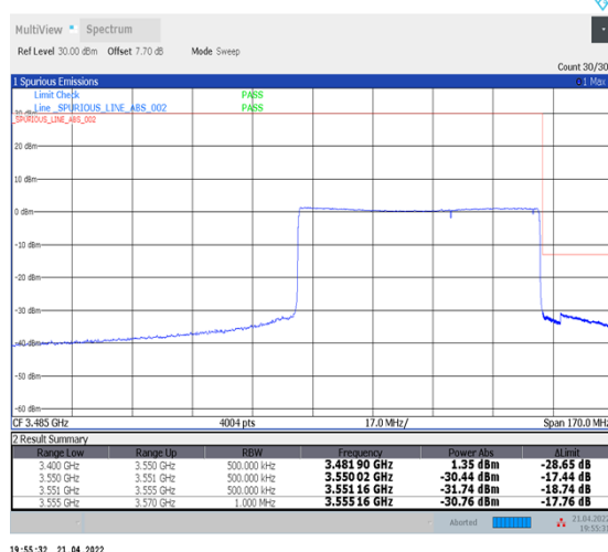
1-N78-3450-3550--30-70-H-6-CP-QPSK-Outer_Full-189@0-Ant1-PASS-see graph
