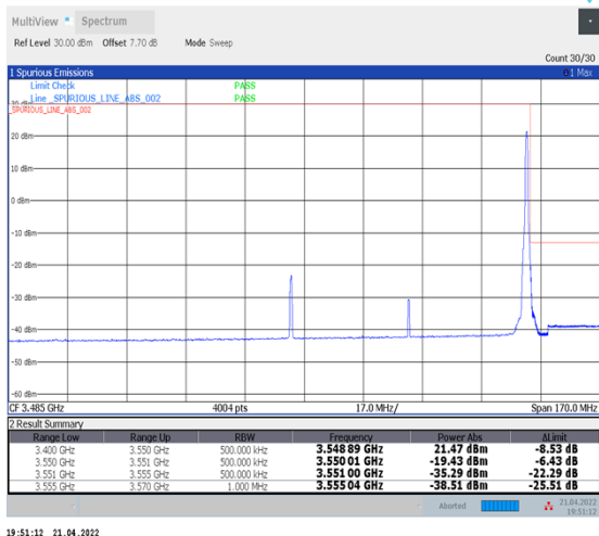
1-N78-3450-3550--30-70-H-2-DFT-PI2BPSK-Edge_1RB_Right-1@188-Ant1-PASS-see graph
