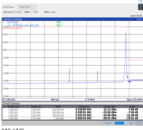
1-N78-3450-3550--30-70-H-5-CP-QPSK-Edge_1RB_Right-1@188-Ant1-PASS-see graph
